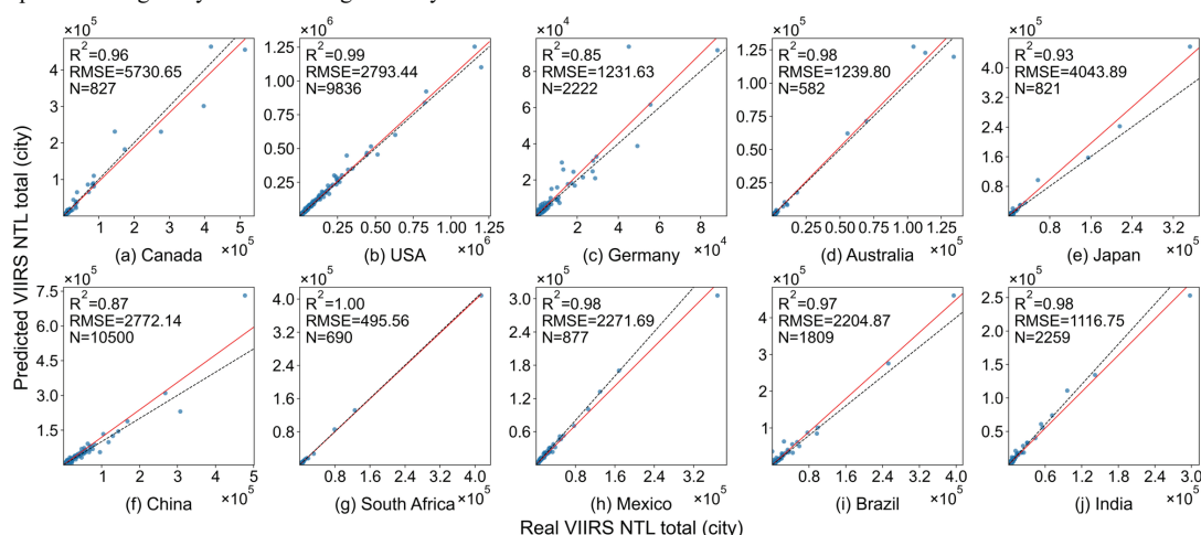
520 Figure 13. City-level scatter density plot of predicted and NPP-VIIRS NTL values for 10 selected countries in 2012-04 (unit: \text{nW cm}^{-2} \text{sr}^{-1} ).
