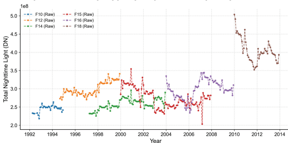
Figure 1. Gap-filled monthly DMSP-OLS NTL data.
