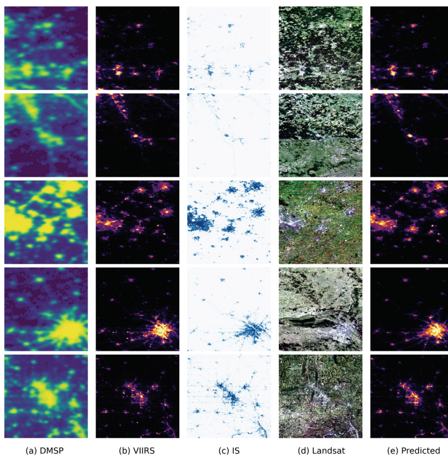
450 Figure 7. Visual comparison of NTL across typical regions in 2013 using the test set. (a) DMSP; (b) VIIRS; (c) Impervious surface; (d) Landsat; (e) Predicted VIIRS-like output.
