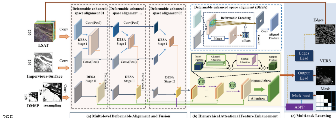
Figure 5. The NightNet framework.
