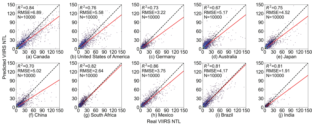
505 Figure 12. Pixel-level scatter density plot of predicted and NPP-VIIRS NTL values for 10 selected countries in 2012-12 (unit: \text{nW cm}^{-2} \text{sr}^{-1} ).
