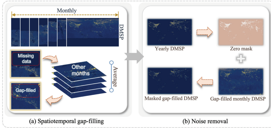
Figure 3. Processing workflow of spatiotemporal gap-filling and denoising.
