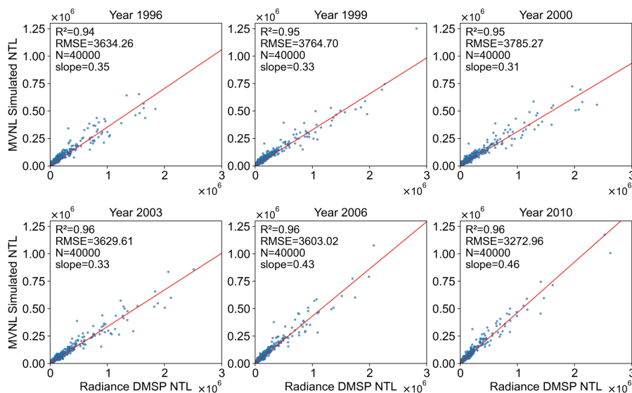
Figure 16. Comparison between radiance-calibrated DMSP-OLS NTL and our extended NPP-VIIRS-like NTL (unit: \text{nW cm}^{-2} \text{sr}^{-1} ) at the city level for (a) 1996, (b) 1999, (c) 2000, (d) 2003, (e) 2006, and (f) 2010.
