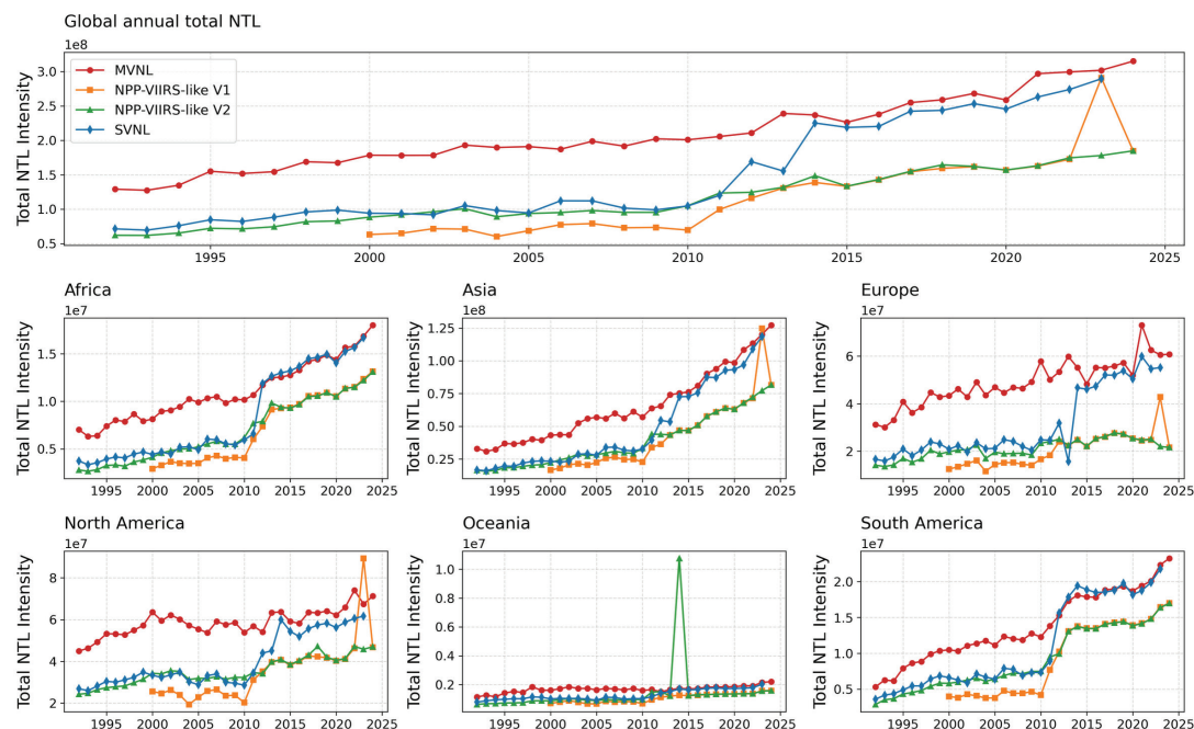
Figure 22. Annual NTL intensity trends from reconstructed VIIRS-like data (1992-2024).
