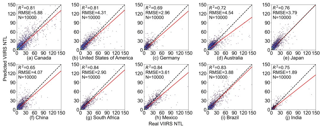
Figure 11. Pixel-level scatter density plot of predicted and NPP-VIIRS NTL values for 10 selected countries in 2012-04 (unit: \text{nW cm}^{-2} \text{sr}^{-1} ).
