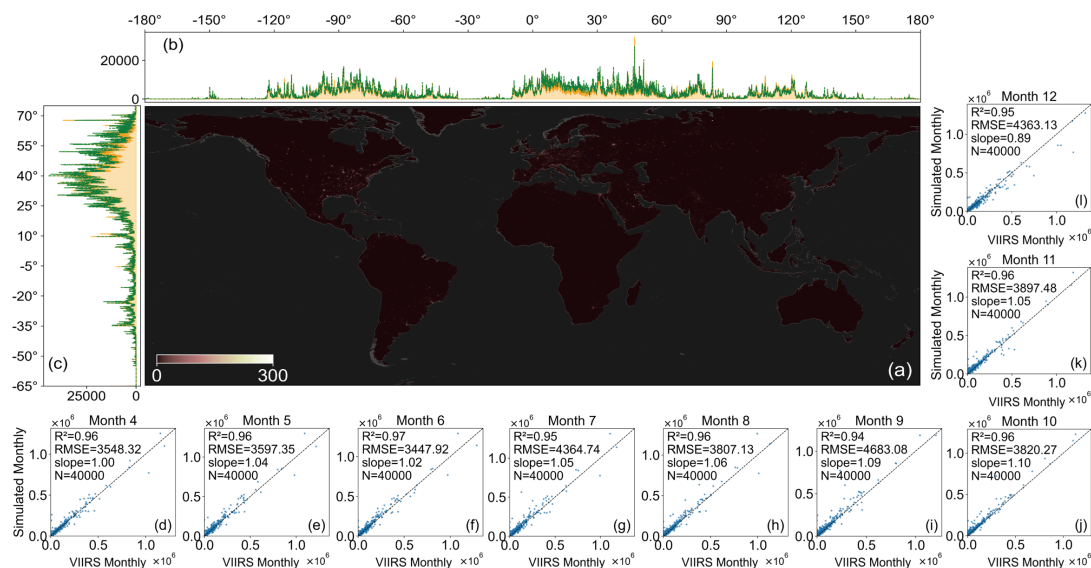
Figure 8. The simulated VIIRS-like data. (a) The generated global NTL intensity in 2012. (b) The longitudinal and (c) latitudinal sum of VIIRS NTL (orange) and Predicted VIIRS (green) with 1° bin (unit: \text{nW cm}^{-2} \text{sr}^{-1} ). (d) to (l) illustrate the city-level prediction errors of the total monthly VIIRS-like NTL from April to December 2012 at the global scale (unit: \text{nW cm}^{-2} \text{sr}^{-1} ).
