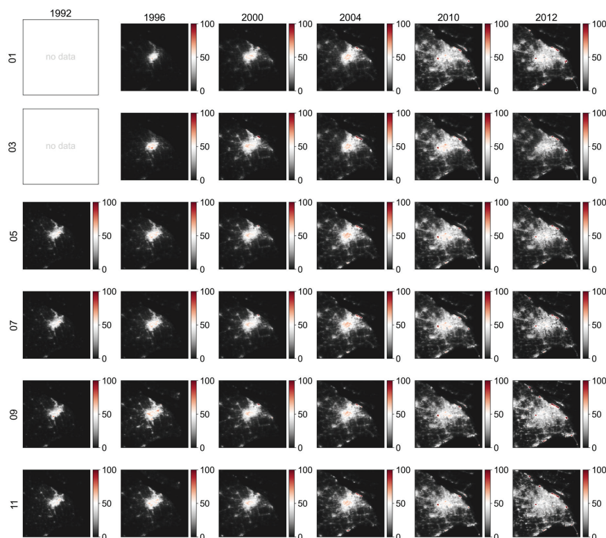
605 Figure 20. Seasonal and interannual spatial patterns of reconstructed VIIRS-like NTL in Shanghai from 1992 to 2012 (unit: \text{nW cm}^{-2} \text{sr}^{-1} ).
