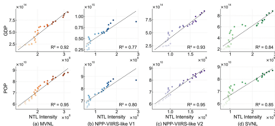
Figure 24. Correlations between annual total NTL intensity and GDP, as well as population, across different datasets.
