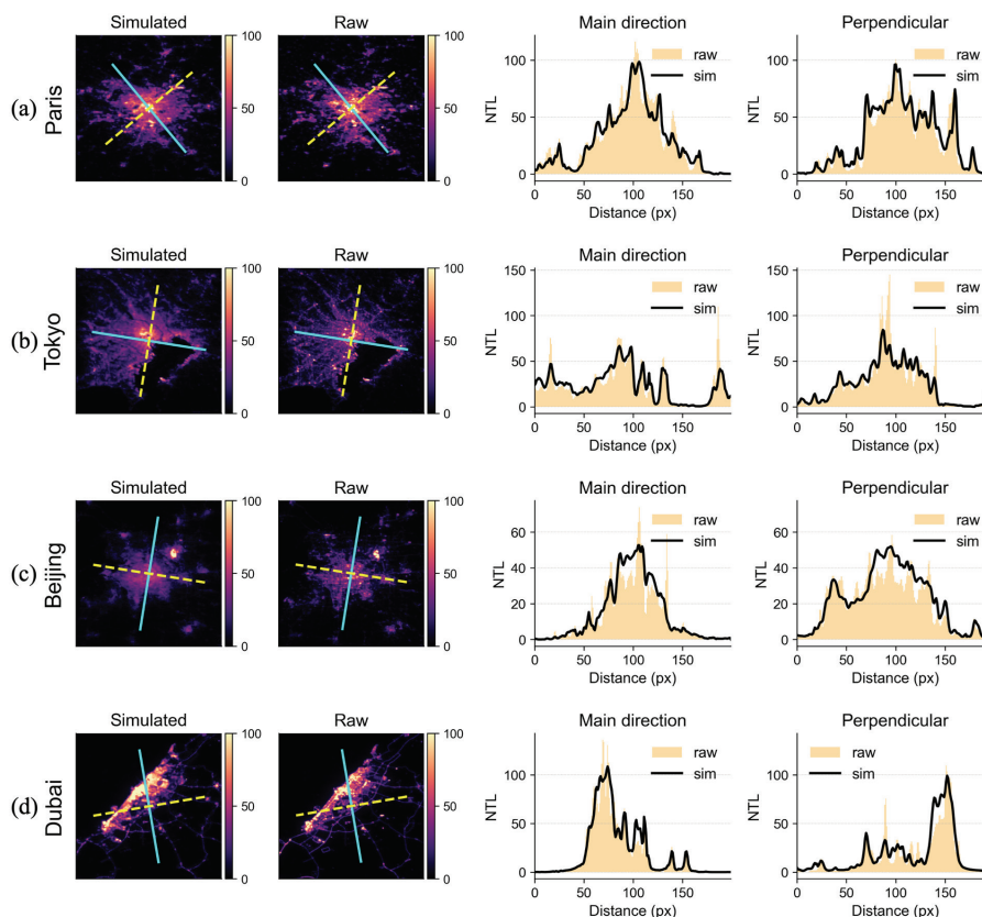
625 Figure 21. Profiles of simulated VIIRS-like and raw NTL intensity (unit: \text{nW cm}^{-2} \text{sr}^{-1} ) in 2012 across (a) Paris, (b) Tokyo, (c) Beijing, and (d) Dubai. The solid cyan line denotes the main direction, while the yellow dashed line represents the perpendicular direction.
