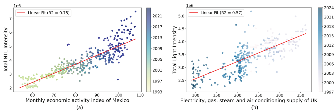
Figure 25. Correlation between total NTL intensity and economic indicators: (a) Monthly economic activity index of Mexico; (b) Electricity, gas, steam, and air conditioning supply index of the UK.
