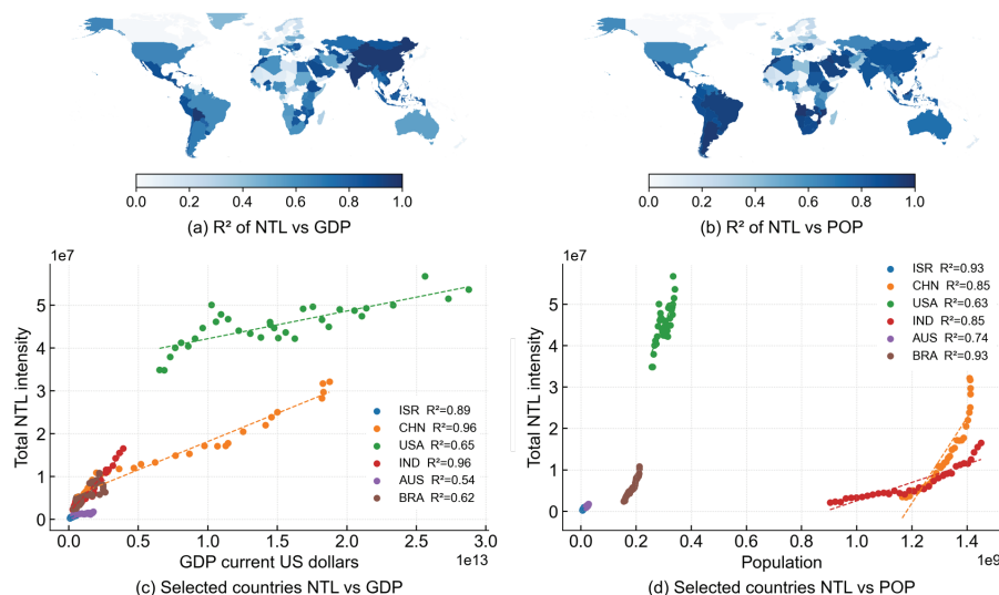
660 Figure 23. Correlation of reconstructed VIIRS-like NTL with GDP and population across global and national scales. (a) national scale R^2 between reconstructed VIIRS NTL and GDP, (b) national scale R^2 between reconstructed VIIRS NTL and population, (c) 665 selected country scatterplots of total NTL versus GDP, and (d) selected country scatterplots of total NTL versus population.
