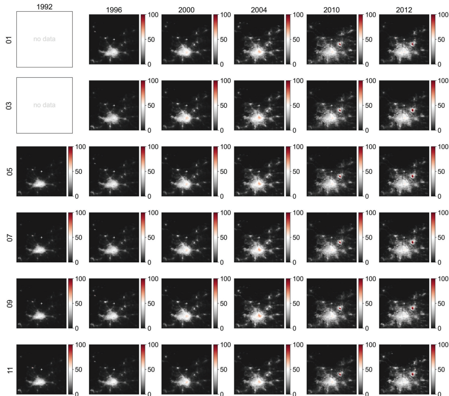
Figure 19. Seasonal and interannual spatial patterns of reconstructed VIIRS-like NTL in Beijing from 1992 to 2012 (unit: \text{nW cm}^{-2} \text{sr}^{-1} ).
