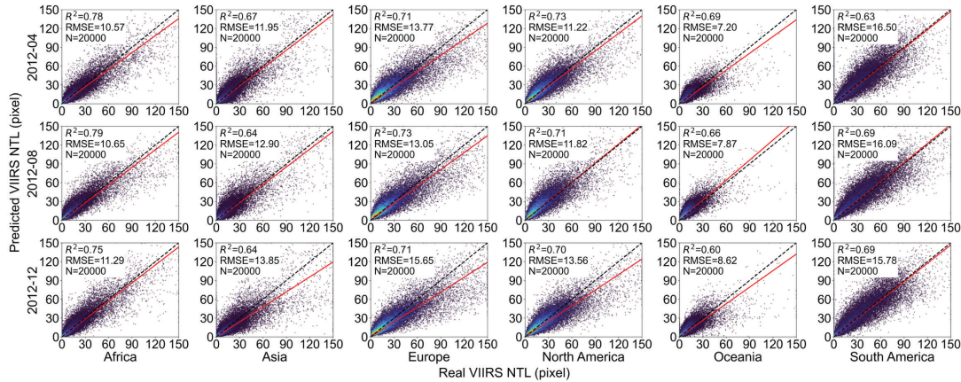
500 Figure 10. Pixel-level scatter density plot comparing simulated VIIRS-like NTL values with NPP VIIRS data across six continents for 2012-04, 2012-08, and 2012-12 (unit: \text{nW cm}^{-2} \text{sr}^{-1} ).
